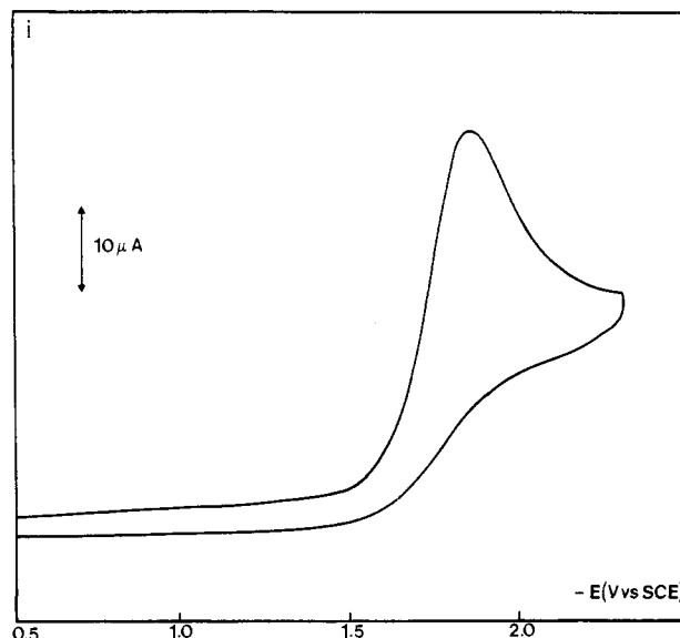
Figure 1. Cyclic voltammety of trans -1,2-dibromocyclohexane (1.35 mM) in DMF (+0.1 M Et 4 NClO 4 ) at a glassy carbon electrode: temperature, 21 °C; sweep rate, 0.1 V·s -1 .
