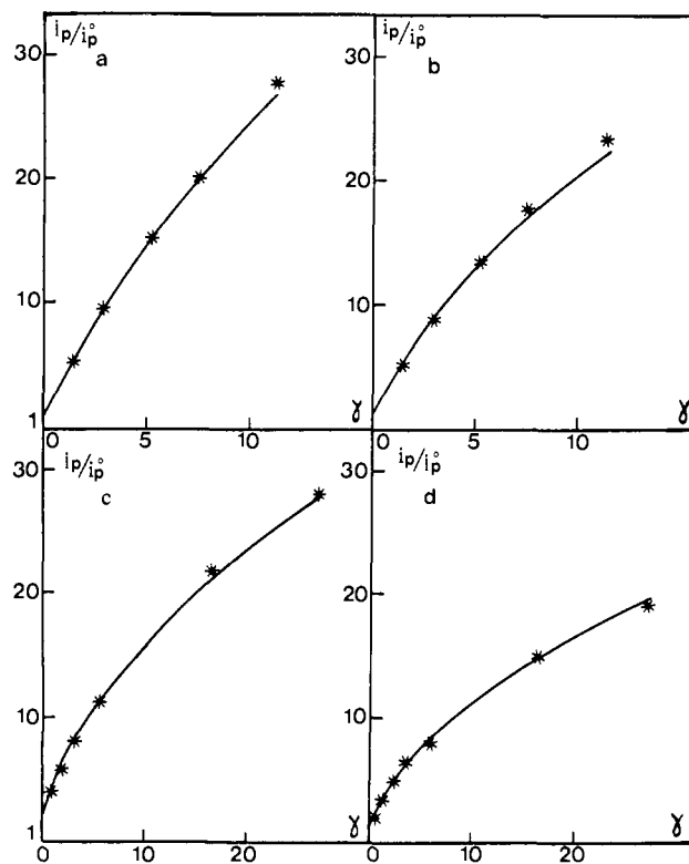
Figure 2. Homogeneous catalysis of the electrochemical reduction of trans -1,2-dibromocyclohexane by the iron(II)/iron(I) couple of OEPFe. Peak current ratio i_p/i_p^0 ( i_p and i_p^0 are the currents, in the presence and absence of DBC, respectively, at a potential equal to the peak potential of the catalyst in the absence of the substrate) as a function of the ratio of the substrate and catalyst concentrations, \gamma : catalyst concentration, 0.98 mM (a, b), 0.214 mM (c, d); sweep rate, 0.1 \text{ V}\cdot\text{s}^{-1} (a, c), 0.2 \text{ V}\cdot\text{s}^{-1} (b, d); temperature, 21^\circ\text{C} ; solvent, DMF + 0.1 \text{ M Et}_4\text{NClO}_4 .
