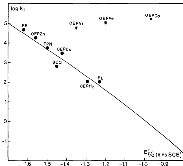
Figure 3. Homogeneous catalysis of the electrochemical reduction of trans -1,2-dibromocyclohexane by aromatic anion radicals and reduced metalloporphyrins. Variation of the rate constant of the rate-determining step with the standard potential E^\circ_{PQ} of the rate-determining step: (●), redox catalysts; (*), chemical catalysts; PE, perylene; TPN, terephthalonitrile; BCQ, benzo[ c ]chinolin; FL, fluorenone; OEP, octaethylporphyrin.
